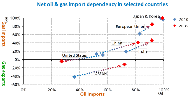
While dependence on imported oil & gas rises in many countries, the United States swims against the tide
