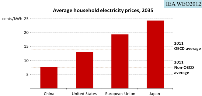
Electricity prices are set to increase with the highest prices persisting in the European Union & Japan, well above those in China & the United States
