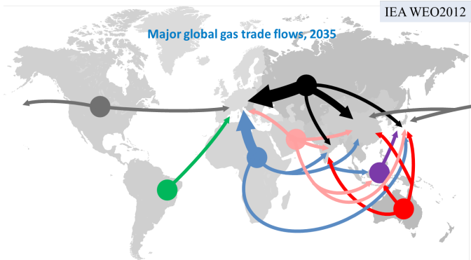
Rising supplies of unconventional gas & LNG help to diversify trade flows, putting pressure on conventional gas suppliers & oil-linked pricing mechanisms
